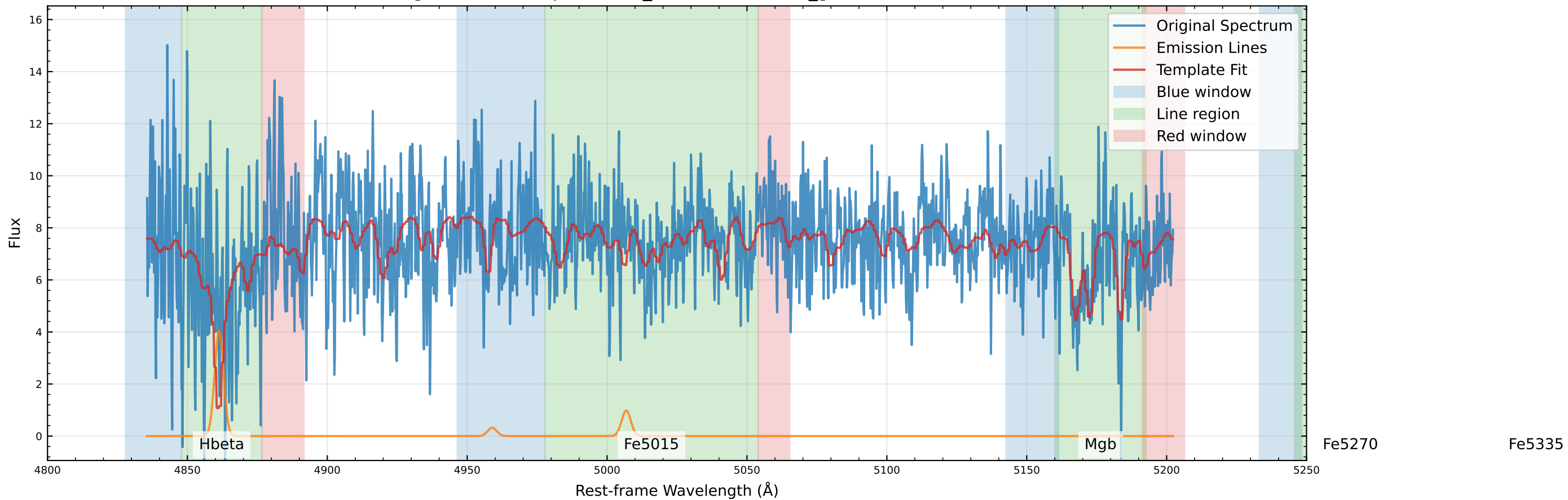
Original Data Comparison ( v_{\text{star}}=-7.6 km/s, v_{\text{gas}}=-57.6 km/s)
