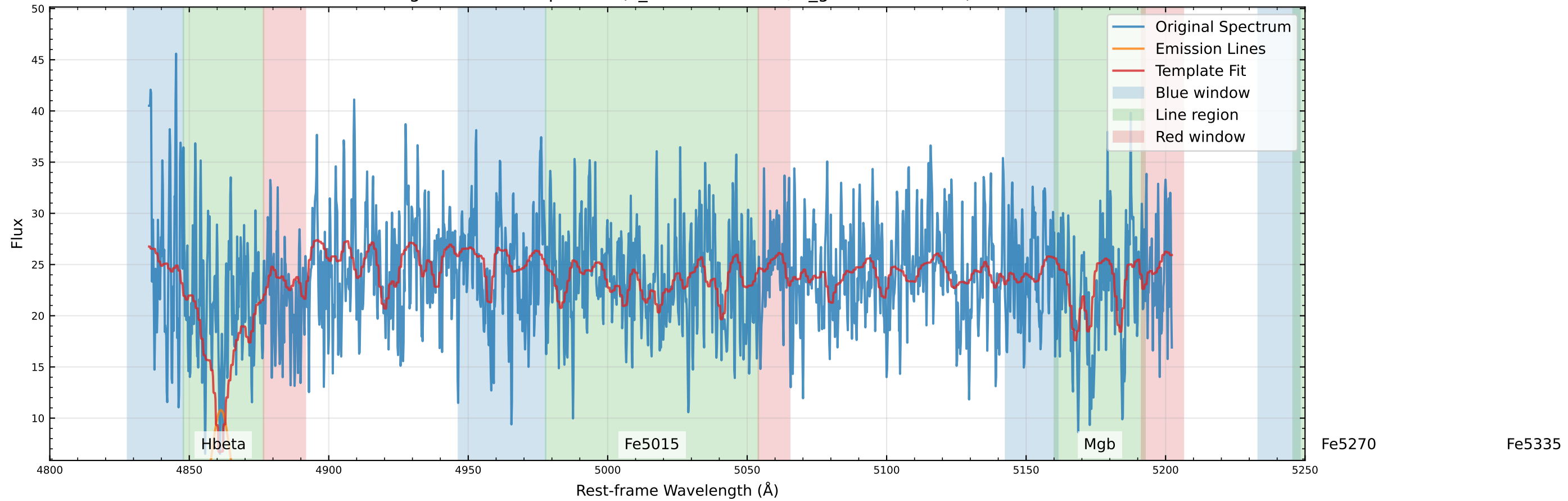
Original Data Comparison (v_star=56.6 km/s, v_gas=112.3 km/s)
