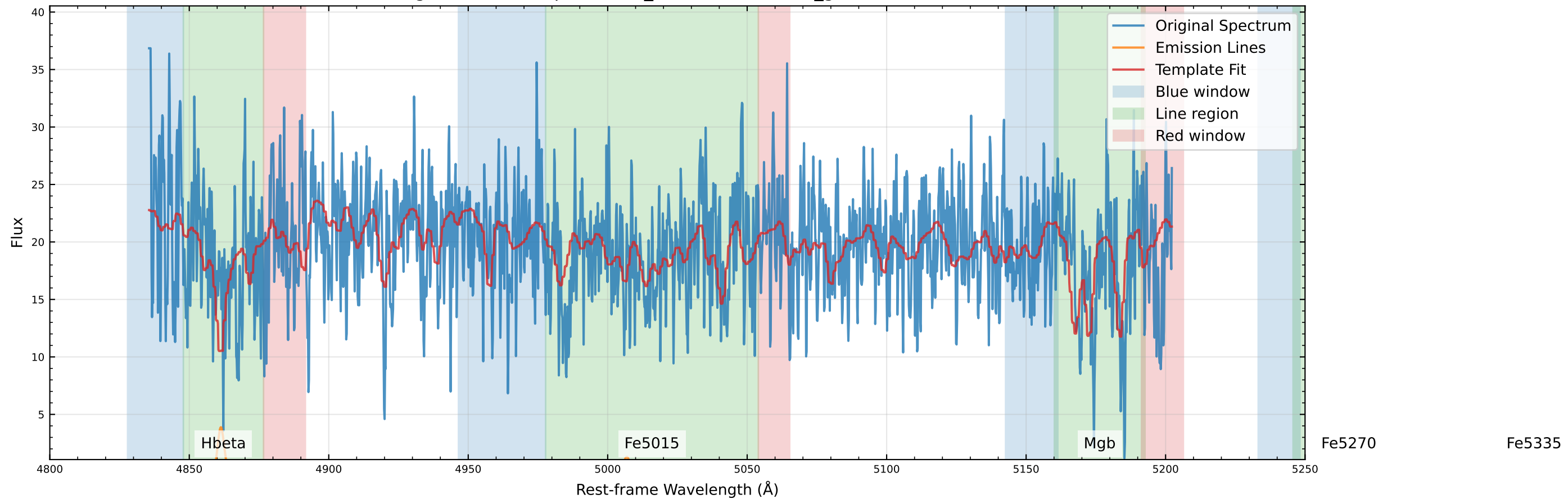
Original Data Comparison (v_star=72.4 km/s, v_gas=67.1 km/s)
