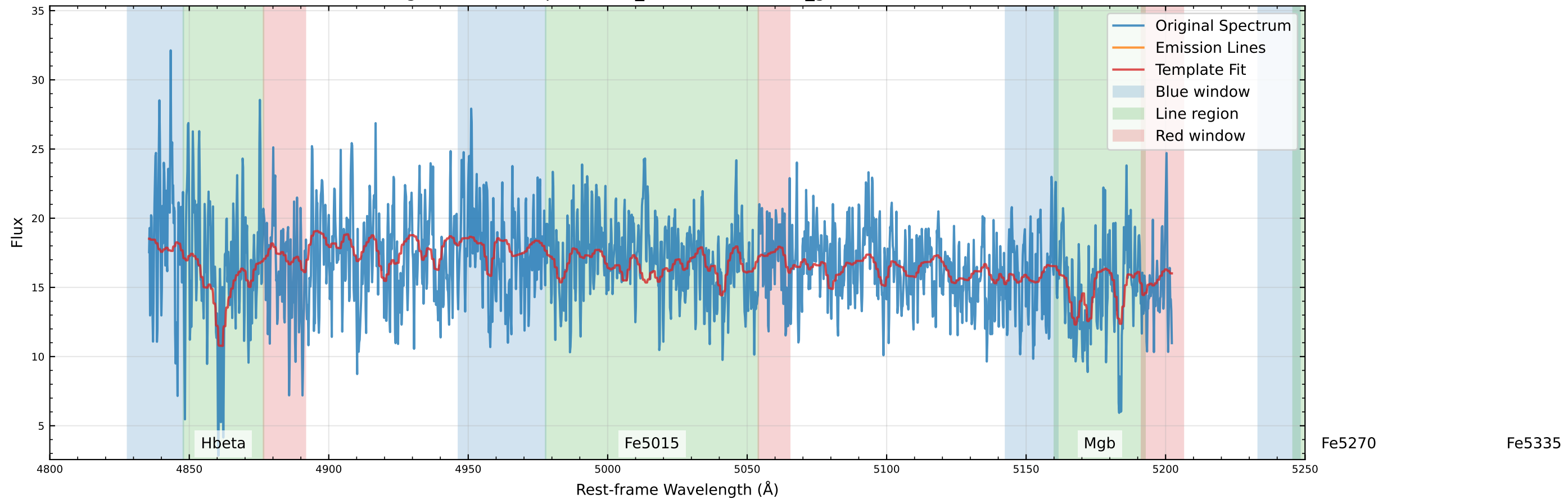
Original Data Comparison (v_star=20.9 km/s, v_gas=-279.1 km/s)
