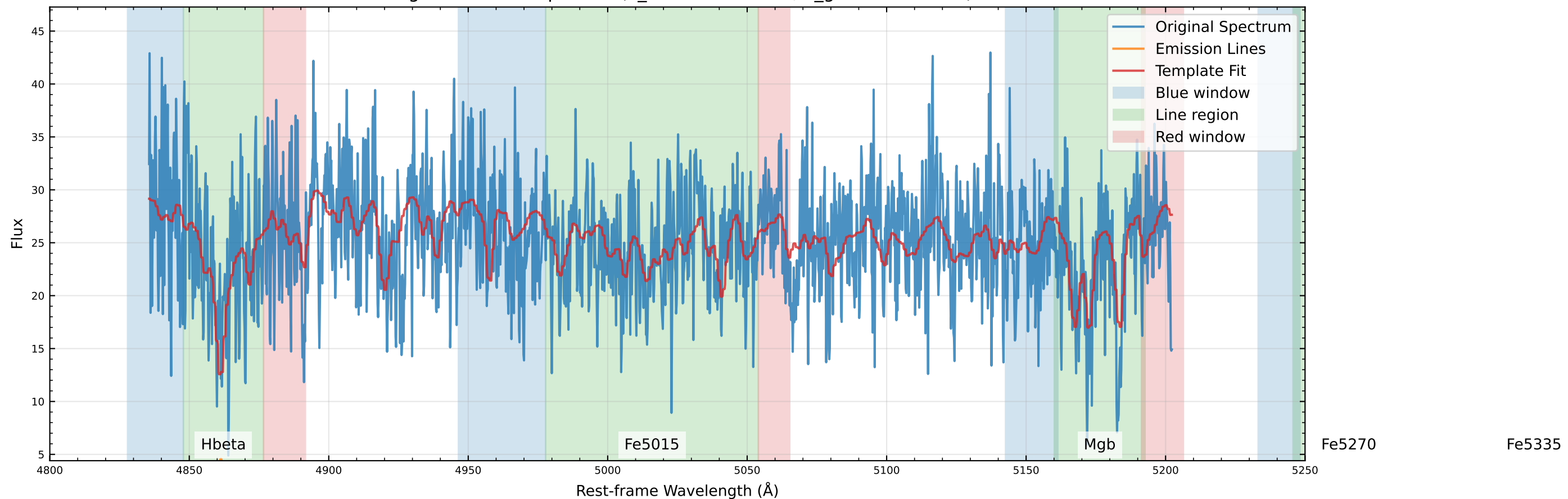
Original Data Comparison (v_star=-17.0 km/s, v_gas=-19.9 km/s)
