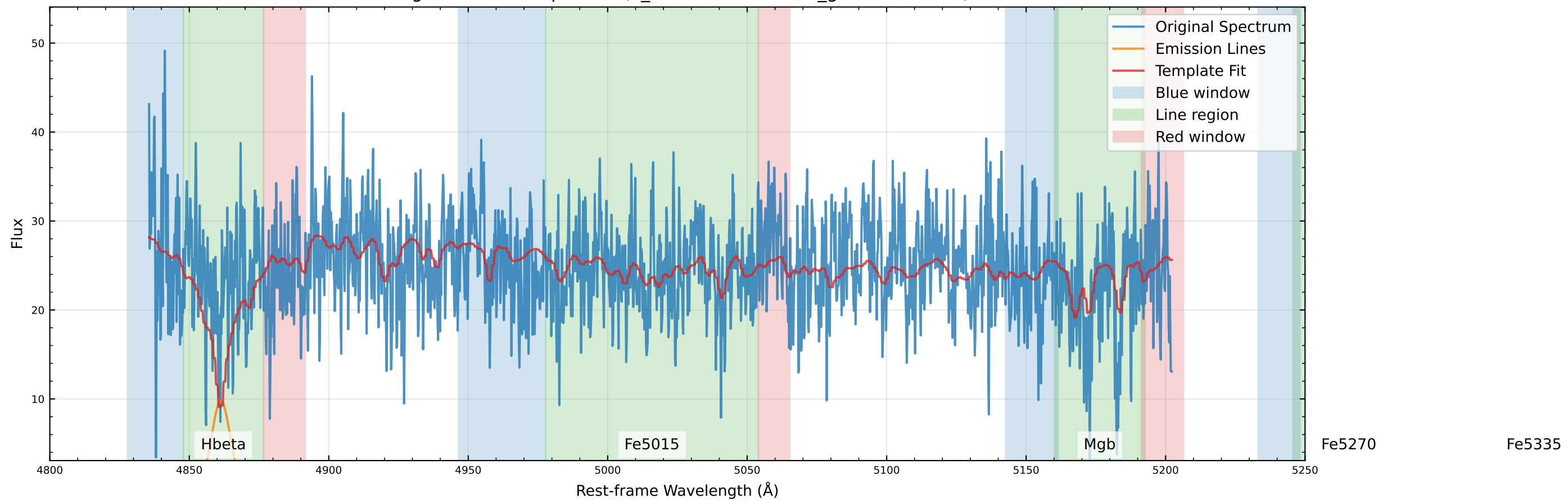
Original Data Comparison (v_star=-24.0 km/s, v_gas=31.8 km/s)
