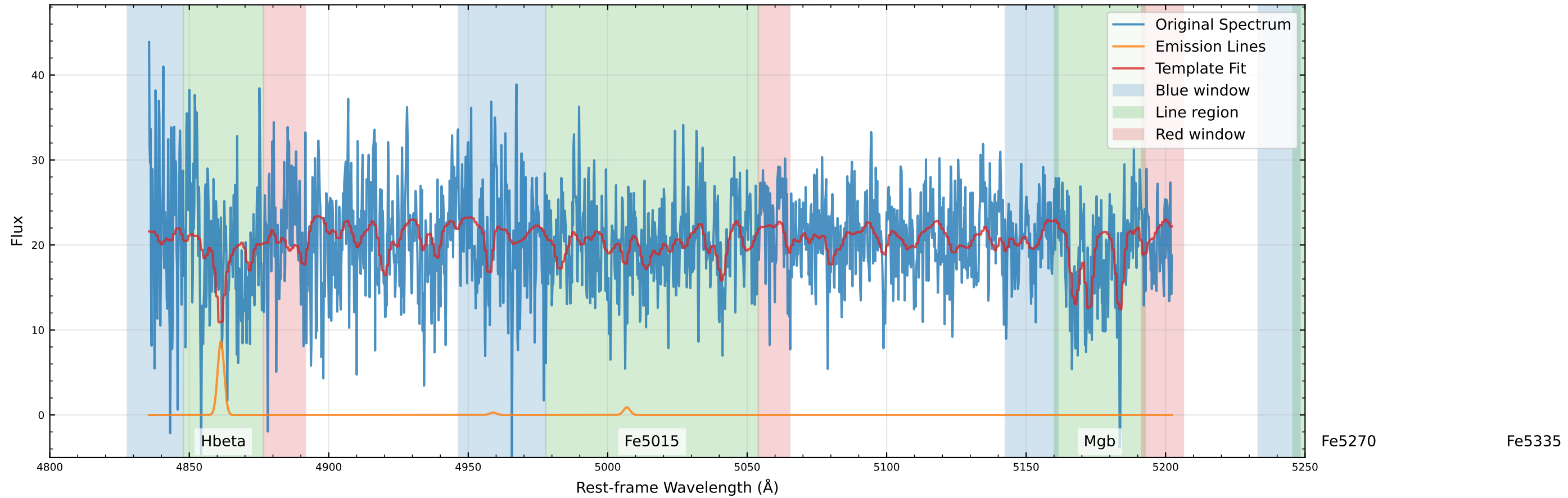
Original Data Comparison (v_star=-1.5 km/s, v_gas=-63.6 km/s)
