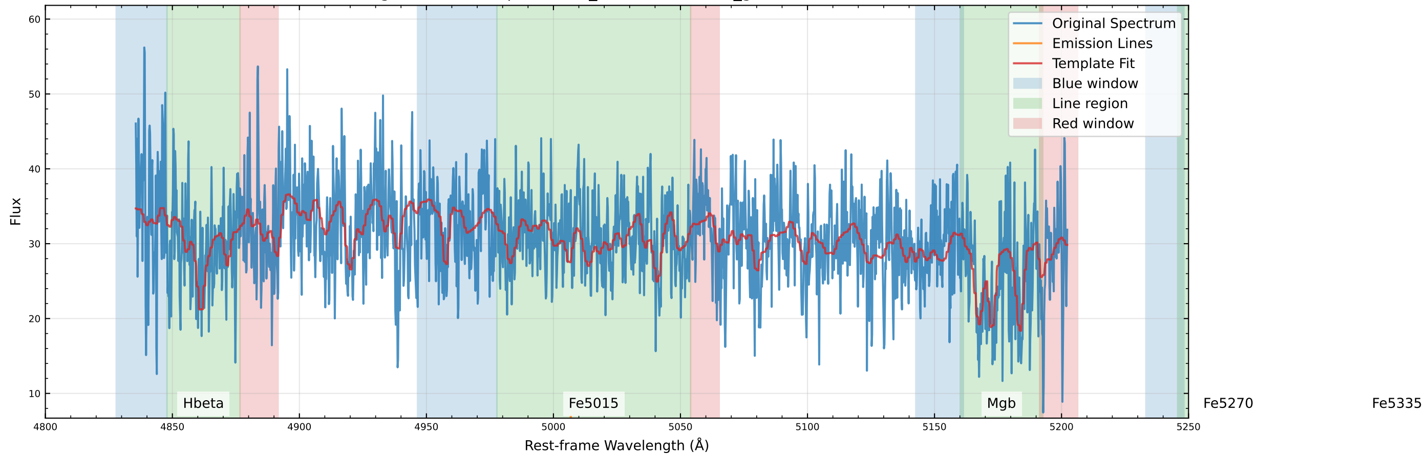
Original Data Comparison (v_star=1.9 km/s, v_gas=-19.4 km/s)
