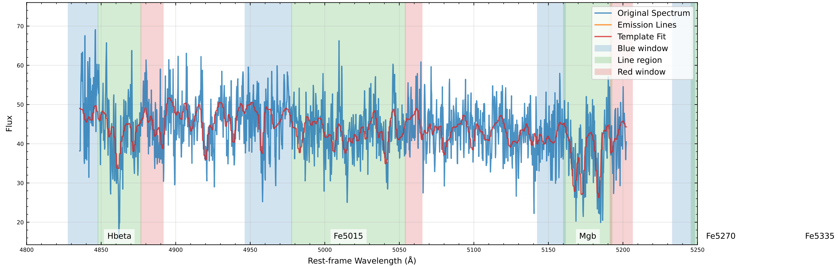
Original Data Comparison (v_star=49.0 km/s, v_gas=162.4 km/s)
