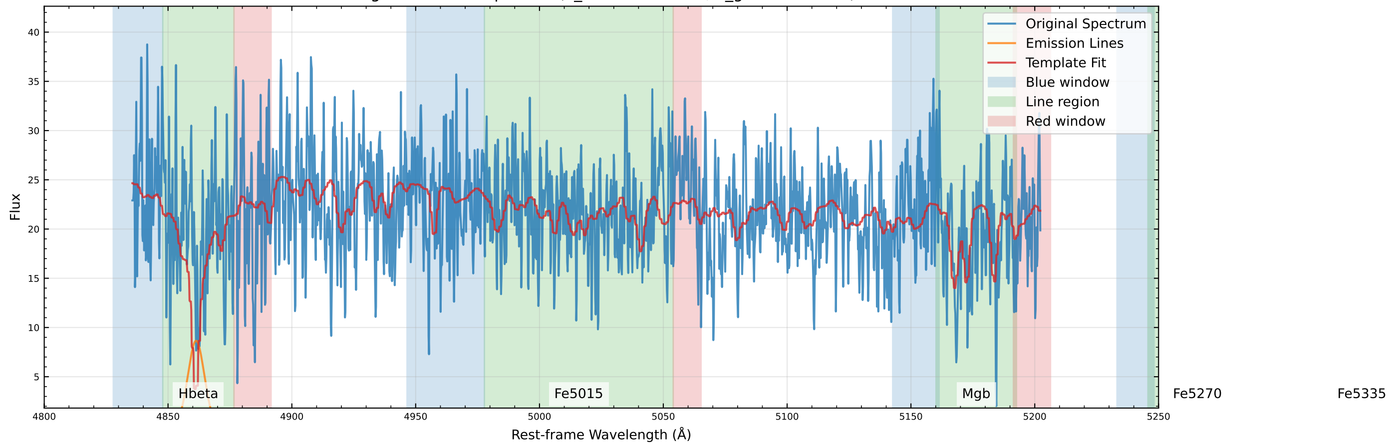
Original Data Comparison (v_star=55.4 km/s, v_gas=-5.9 km/s)
