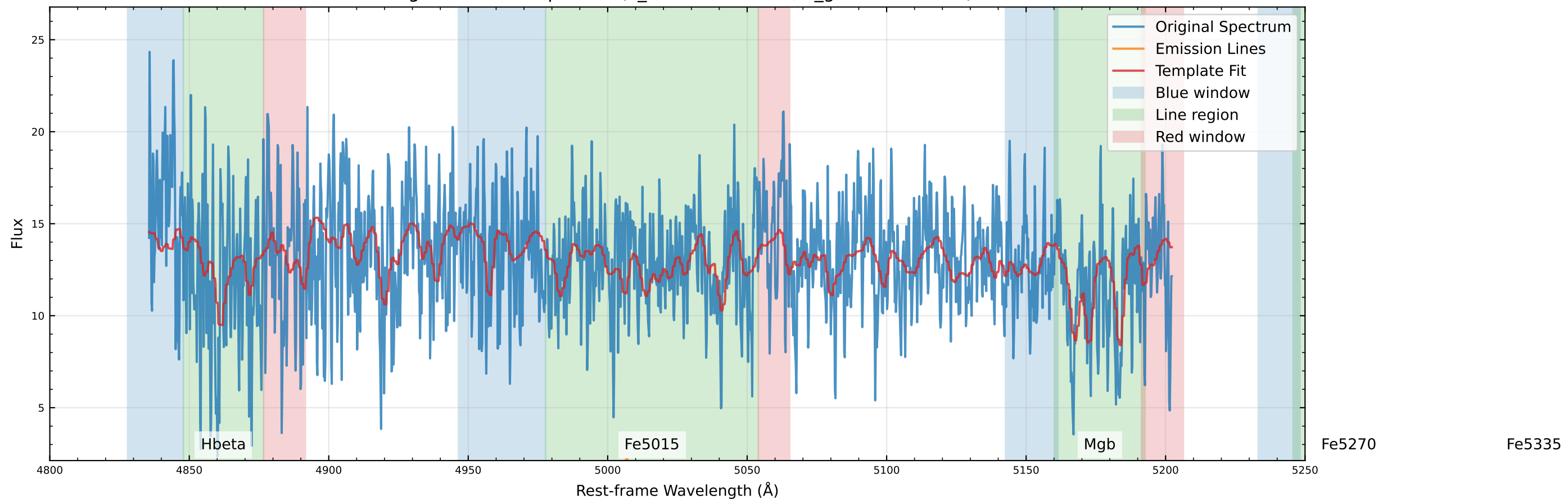
Original Data Comparison (v_star=-52.0 km/s, v_gas=-81.7 km/s)
