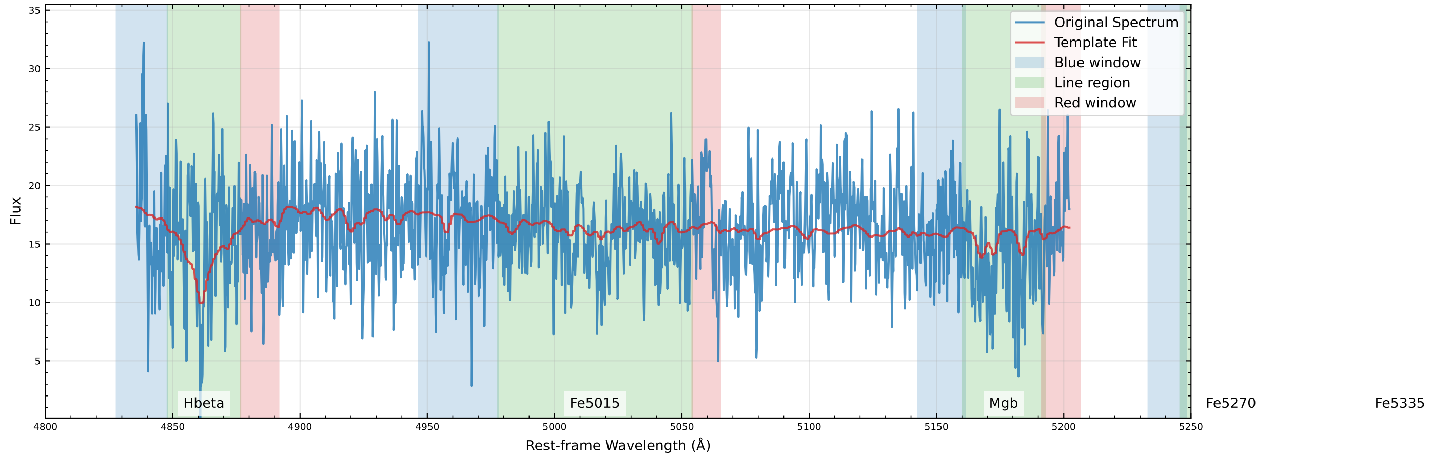
Original Data Comparison ( v_{\text{star}}=-46.6 km/s)
