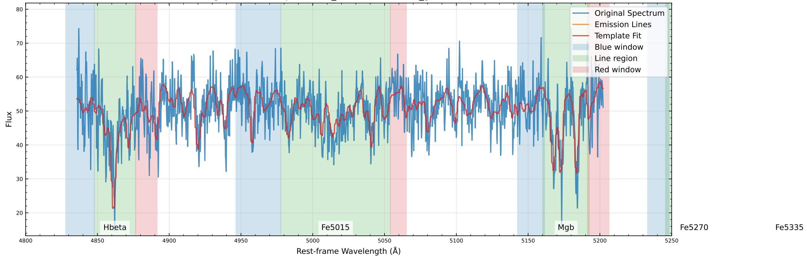
Original Data Comparison (v_star=33.3 km/s, v_gas=42.8 km/s)
