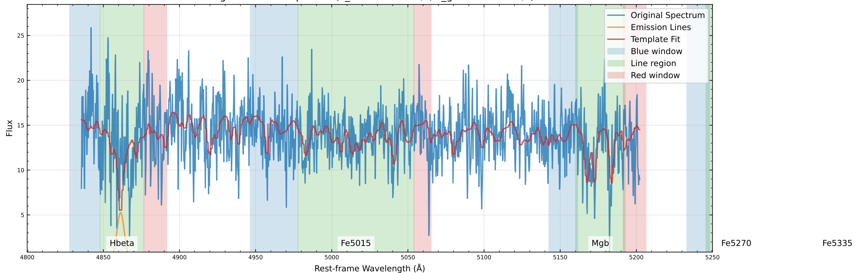
Original Data Comparison (v_star=-44.6 km/s, v_gas=-103.4 km/s)
