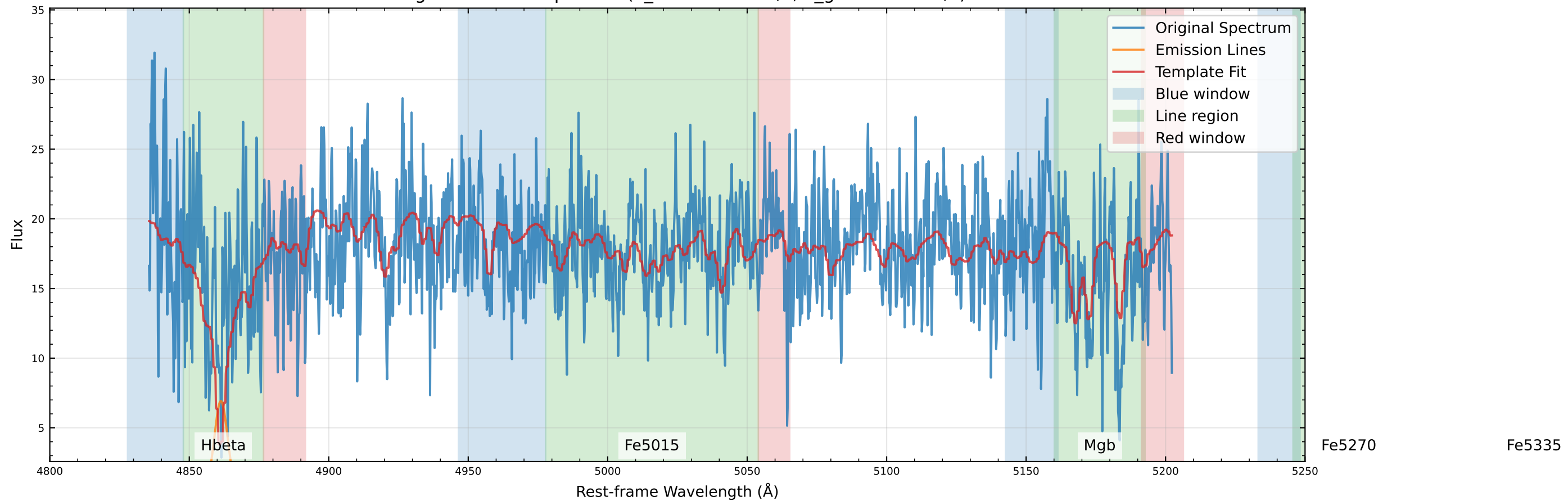
Original Data Comparison (v_star=11.4 km/s, v_gas=60.7 km/s)
