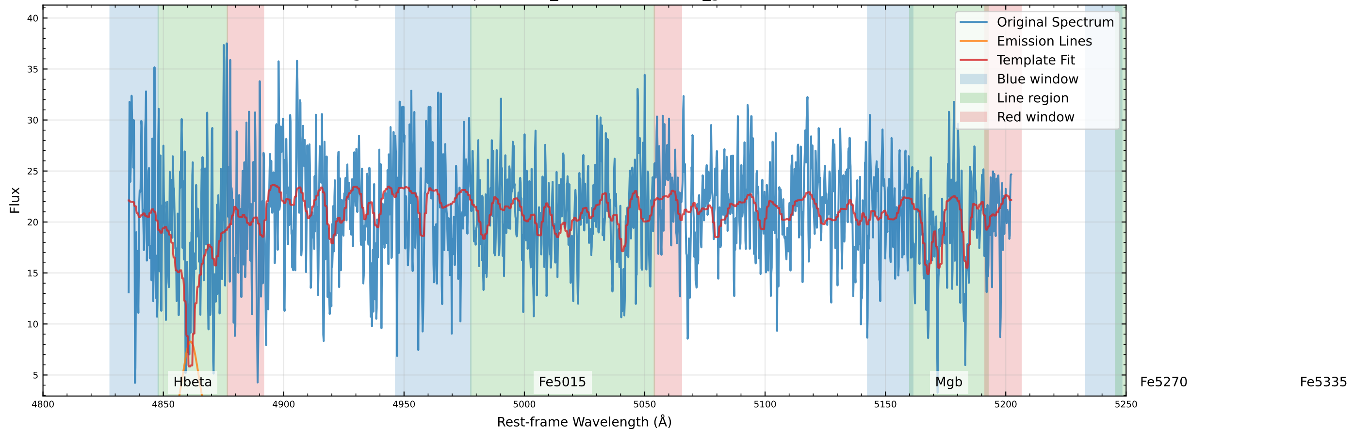
Original Data Comparison (v_star=-16.4 km/s, v_gas=-25.9 km/s)
