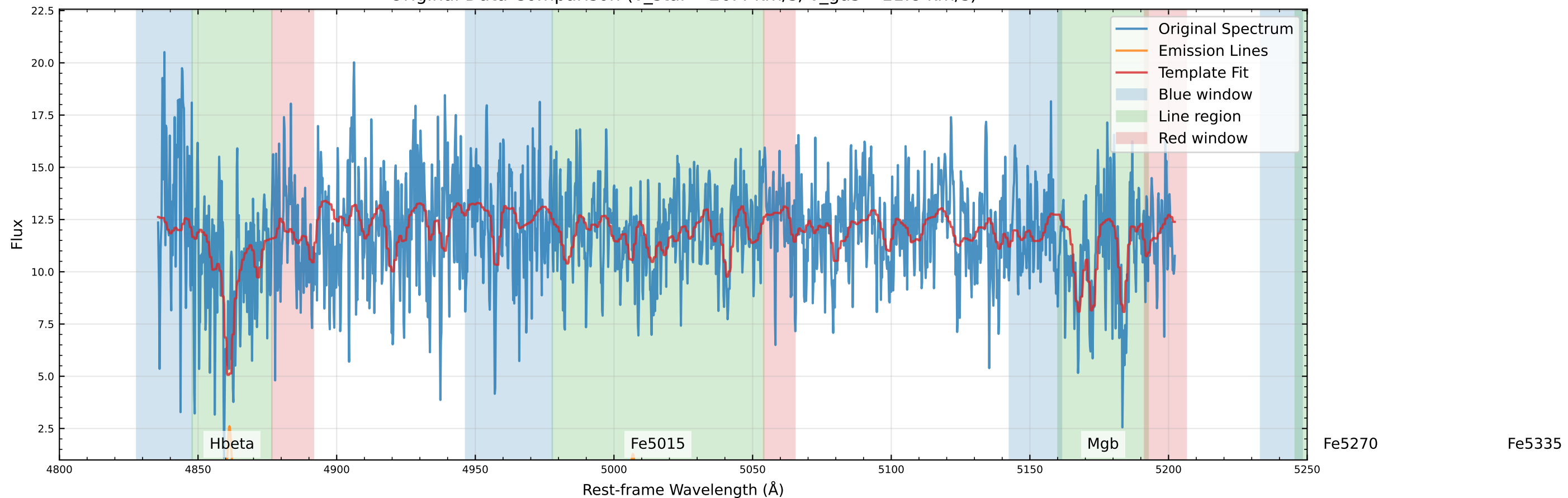
Original Data Comparison (v_star=-26.4 km/s, v_gas=-11.8 km/s)
