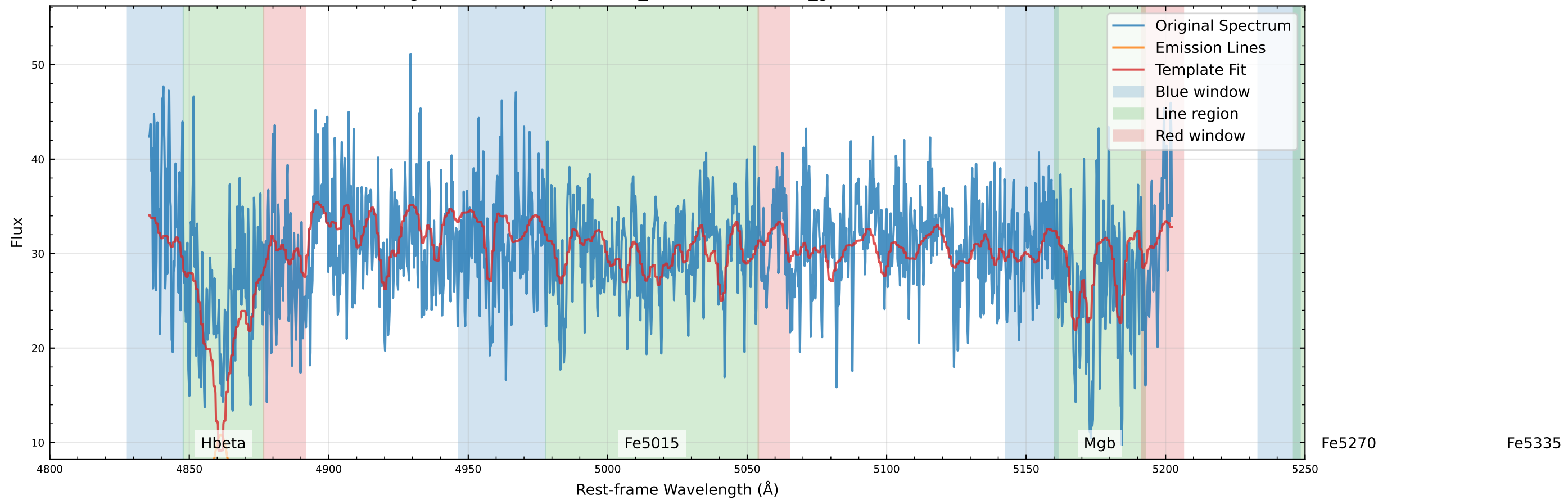
Original Data Comparison (v_star=33.9 km/s, v_gas=106.4 km/s)
