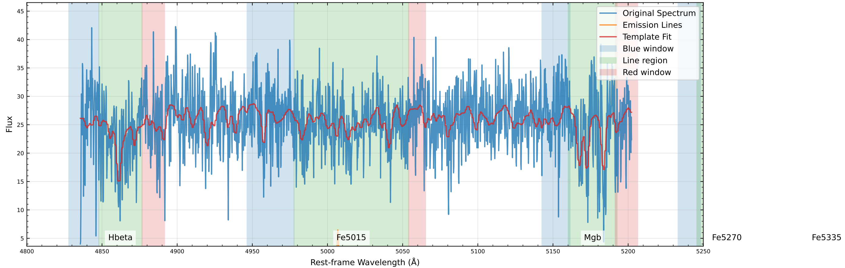
Original Data Comparison (v_star=19.3 km/s, v_gas=-17.8 km/s)
