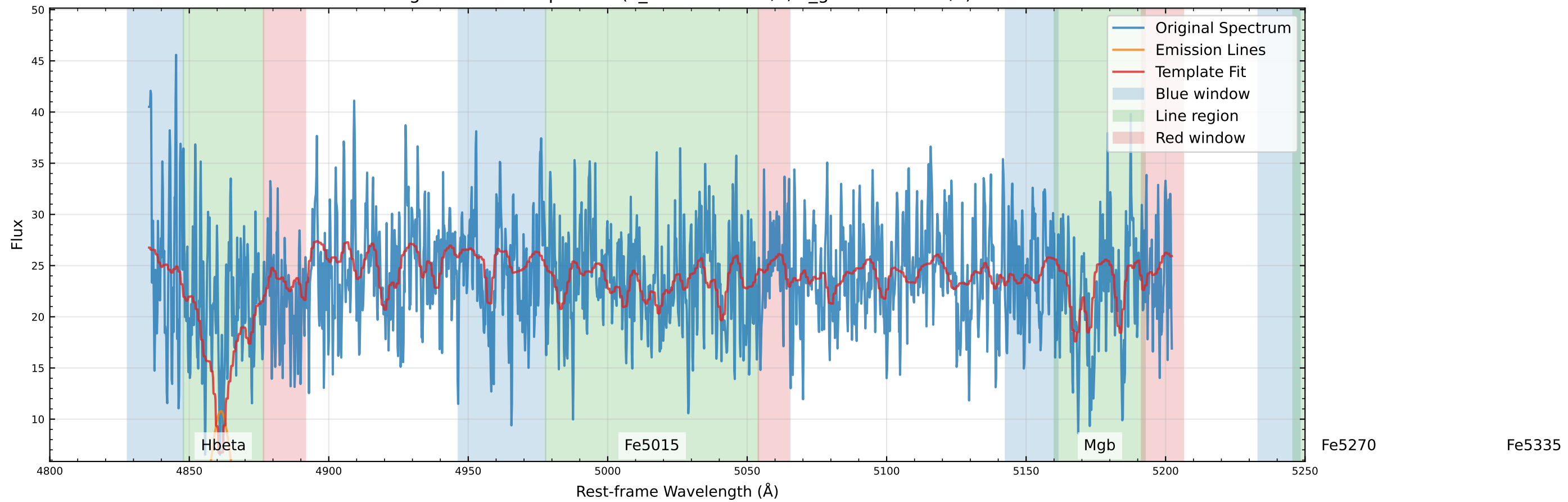
Original Data Comparison (v_star=56.6 km/s, v_gas=112.3 km/s)
