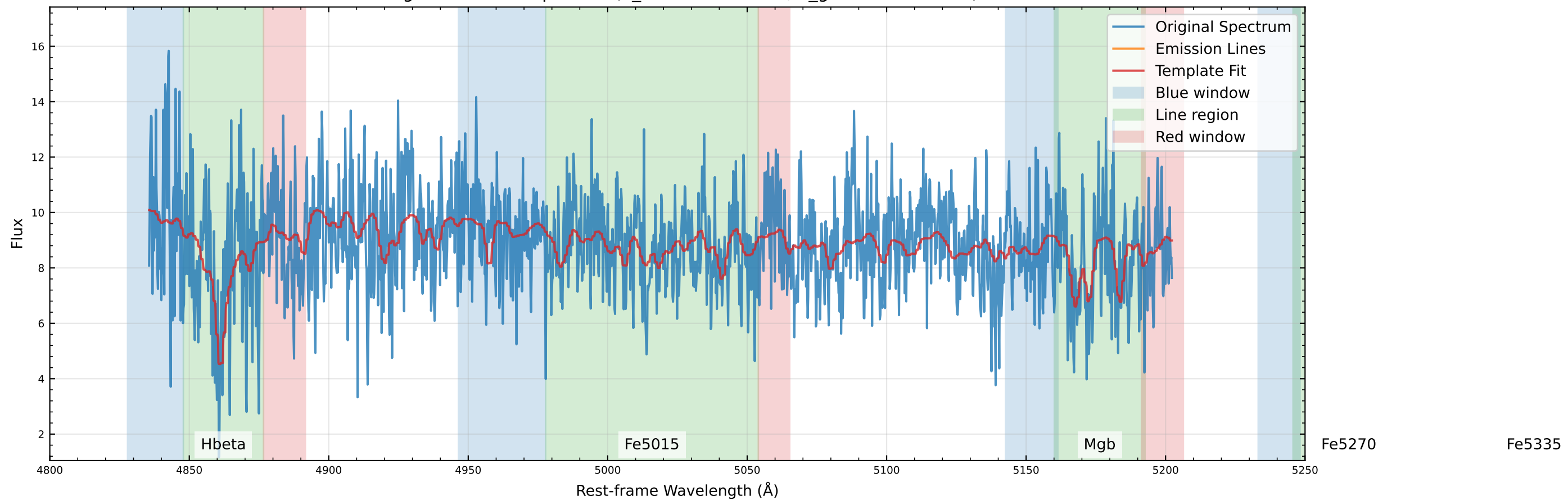
Original Data Comparison (v_star=-27.0 km/s, v_gas=-179.8 km/s)
