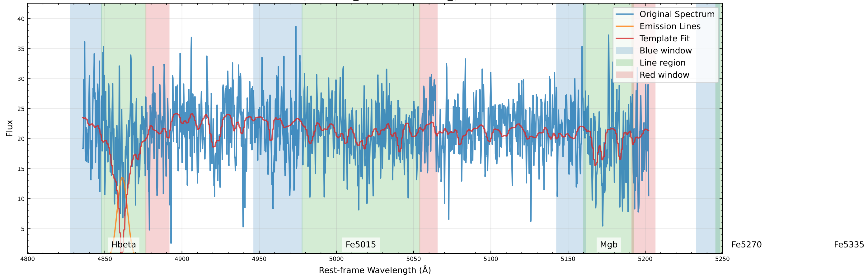
Original Data Comparison (v_star=59.5 km/s, v_gas=134.9 km/s)
