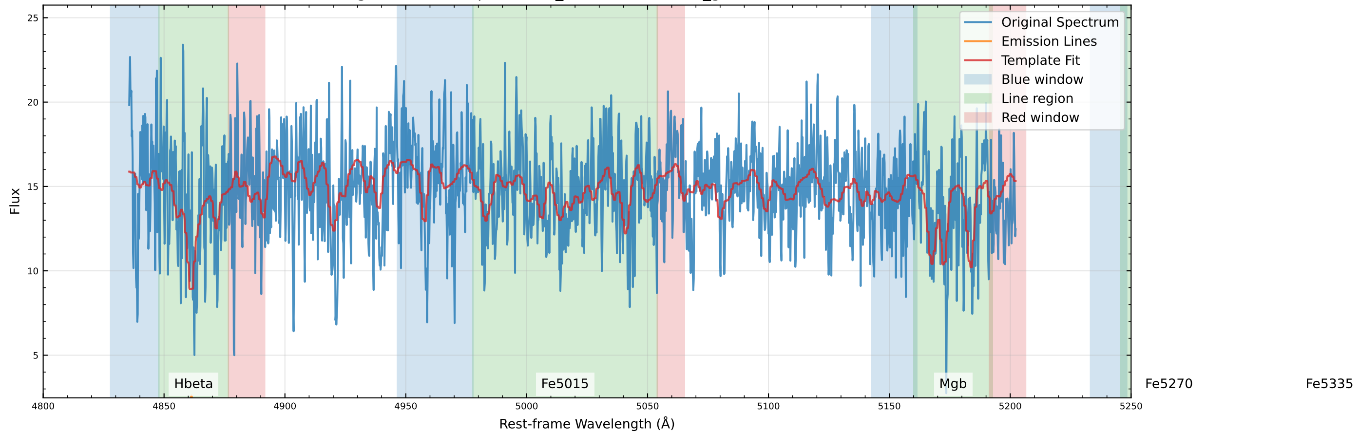
Original Data Comparison (v_star=47.9 km/s, v_gas=-18.0 km/s)
