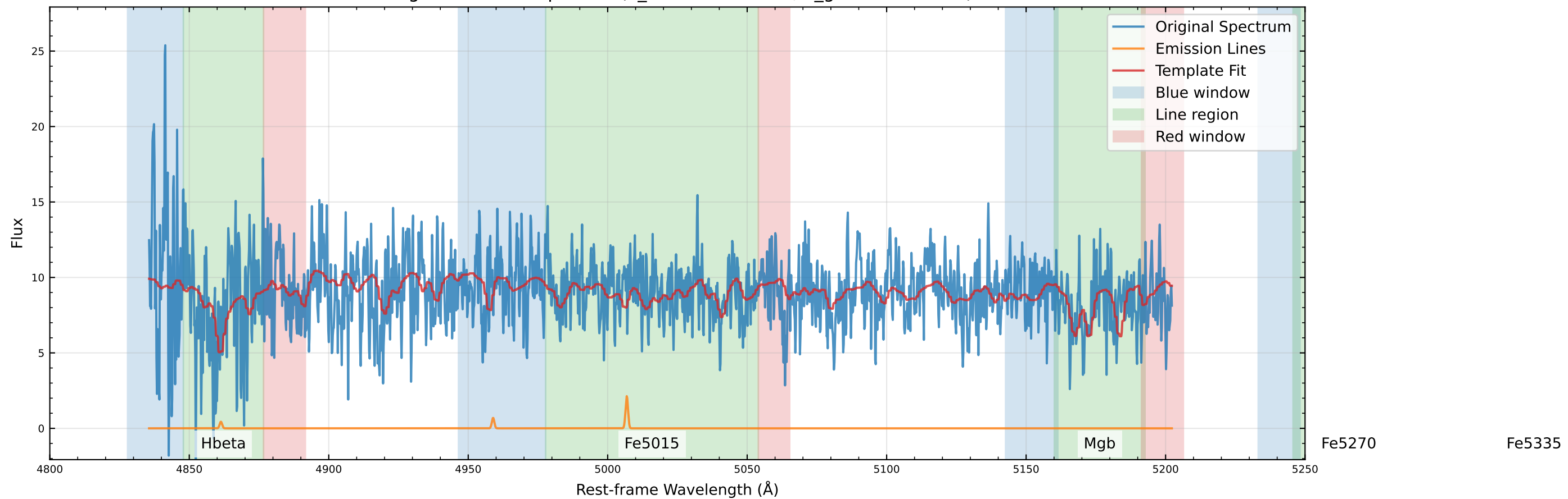
Original Data Comparison (v_star=-73.3 km/s, v_gas=-62.6 km/s)
