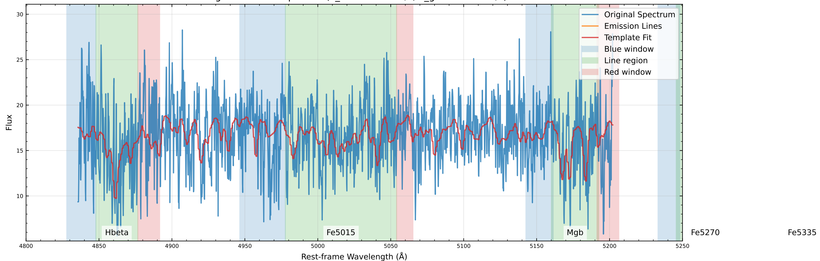
Original Data Comparison (v_star=62.6 km/s, v_gas=-13.2 km/s)
