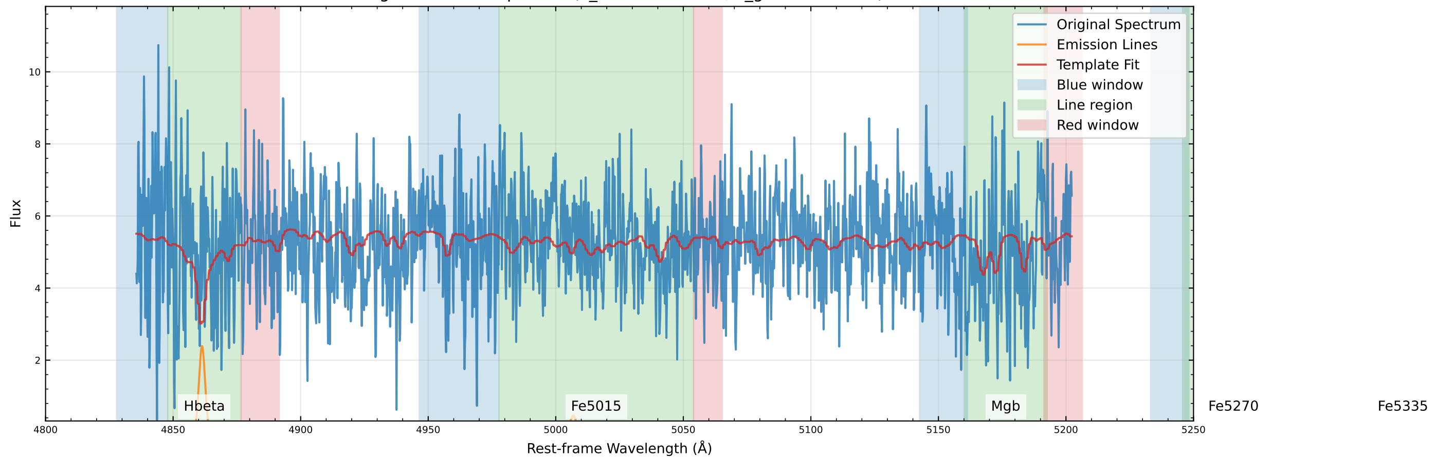
Original Data Comparison (v_star=49.1 km/s, v_gas=61.9 km/s)
