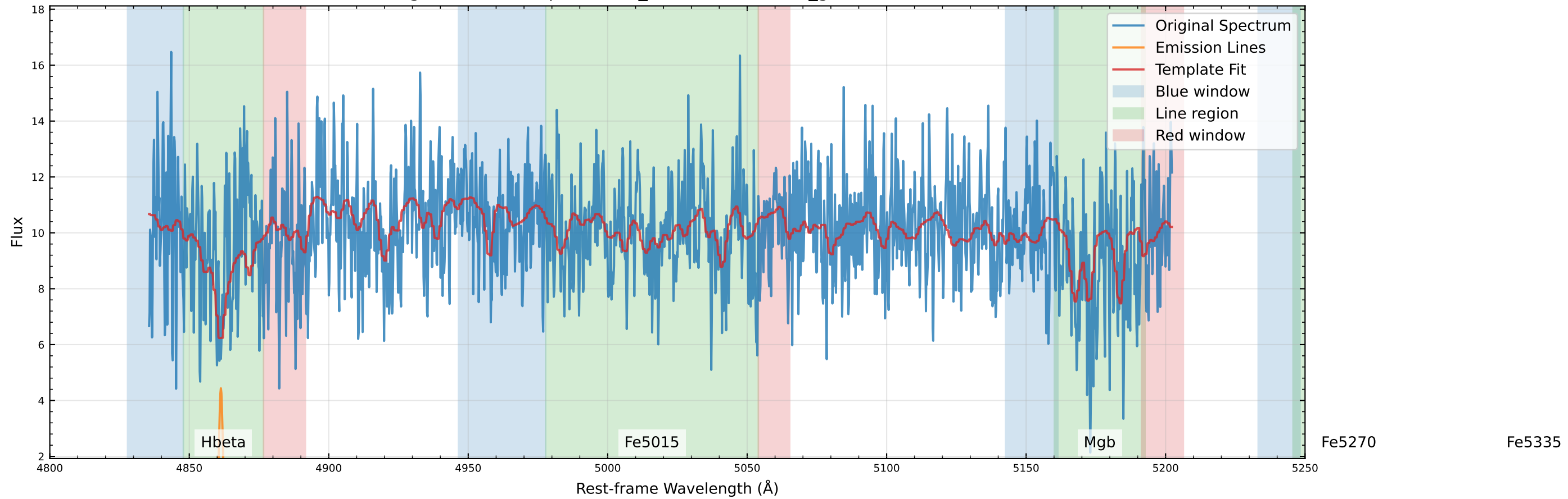
Original Data Comparison (v_star=65.6 km/s, v_gas=110.9 km/s)
