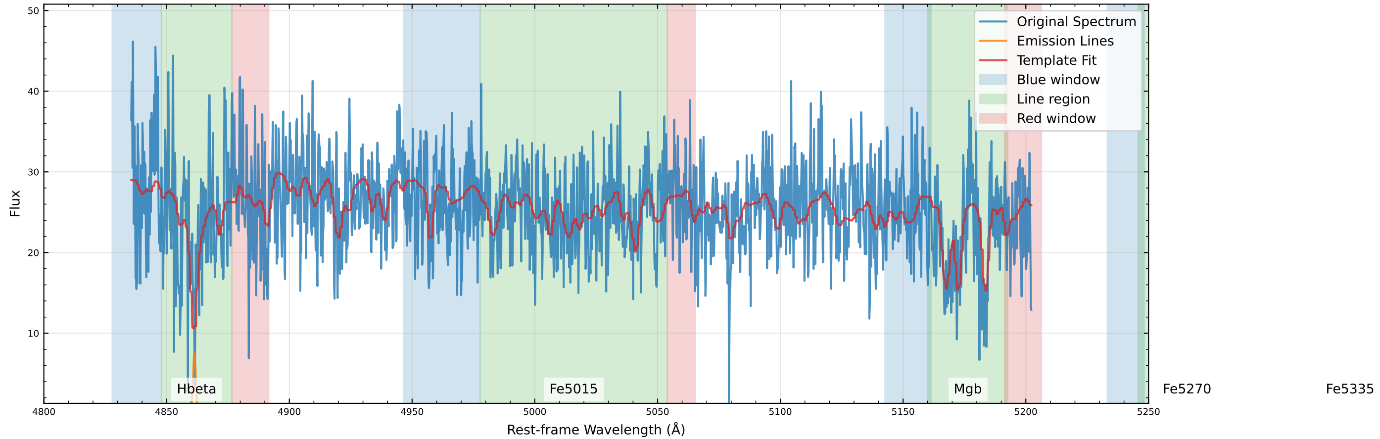
Original Data Comparison (v_star=-20.3 km/s, v_gas=-72.0 km/s)
