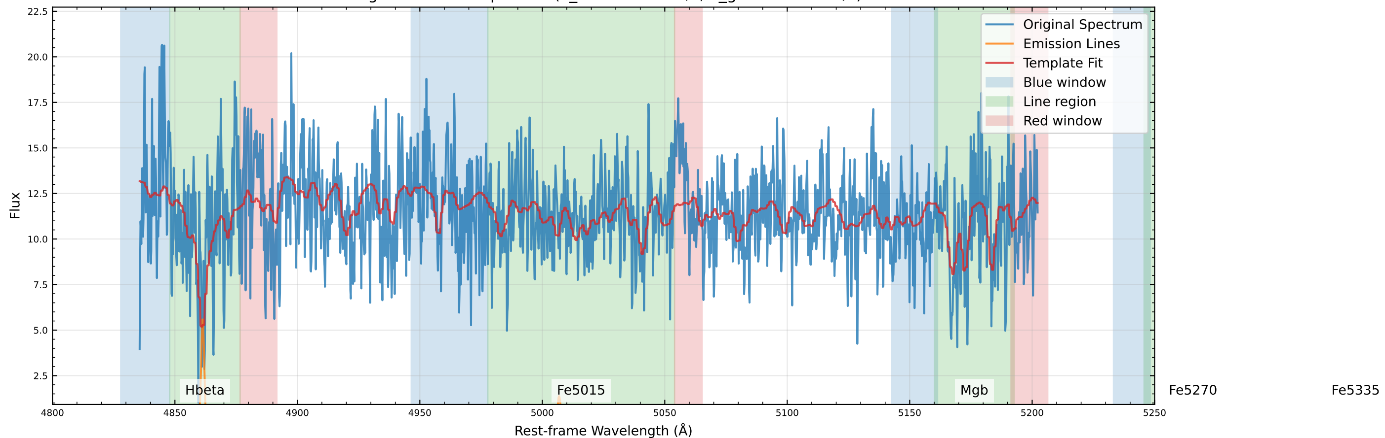
Original Data Comparison (v_star=34.1 km/s, v_gas=118.8 km/s)
