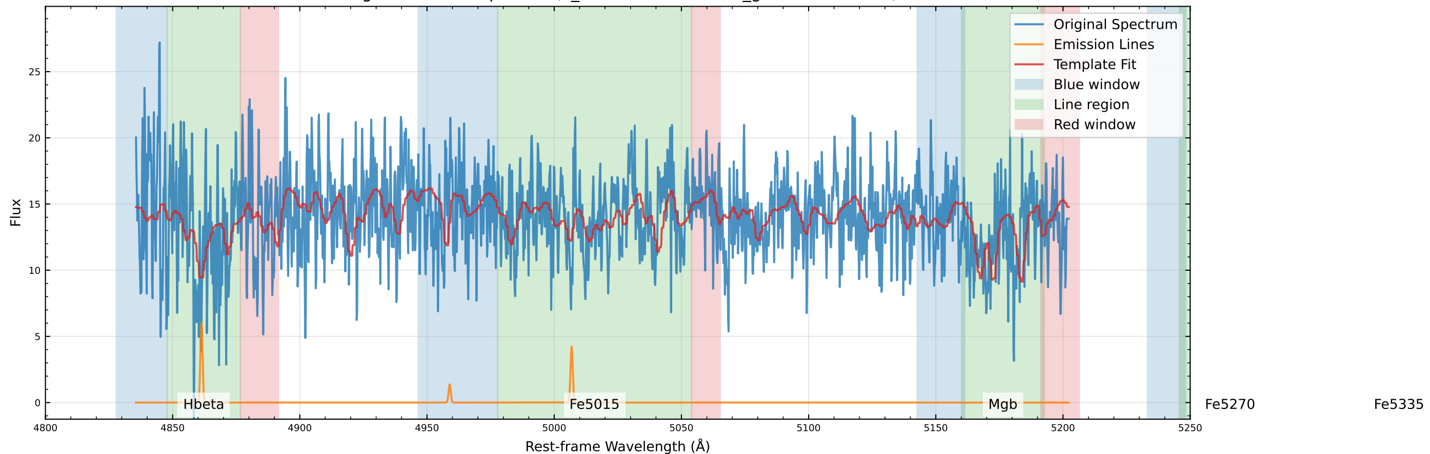
Original Data Comparison (v_star=-120.0 km/s, v_gas=-238.9 km/s)
