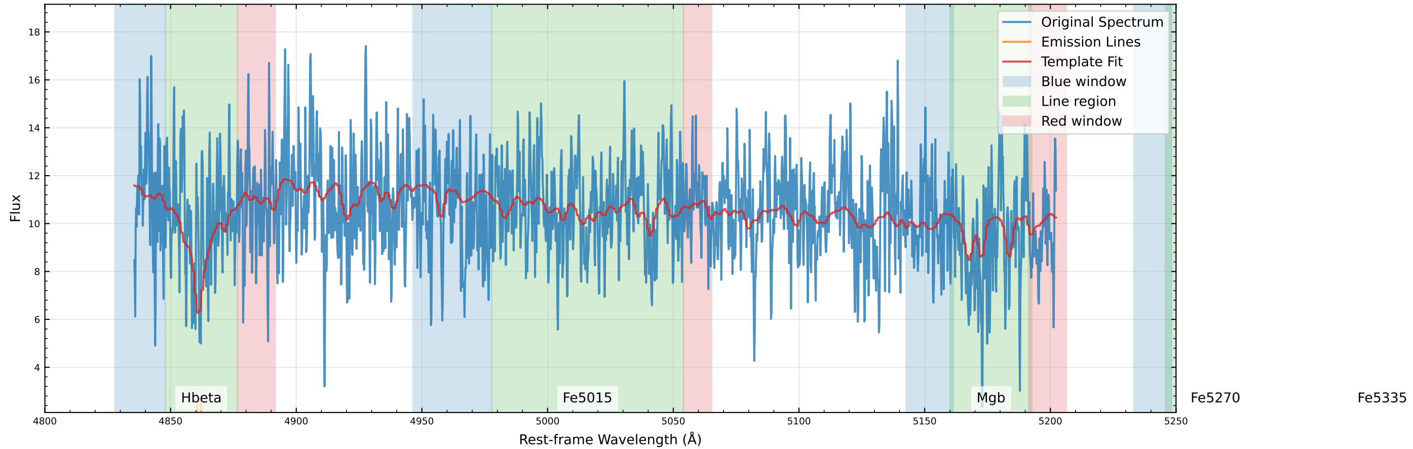
Original Data Comparison (v_star=27.3 km/s, v_gas=49.8 km/s)
