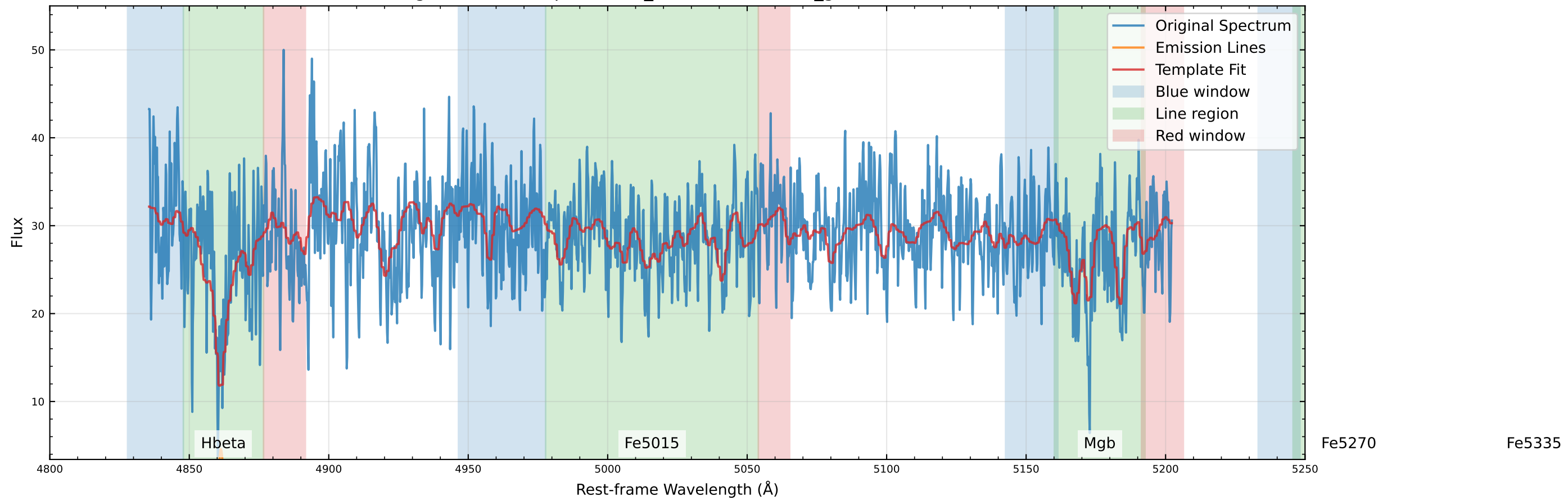
Original Data Comparison (v_star=16.3 km/s, v_gas=23.0 km/s)
