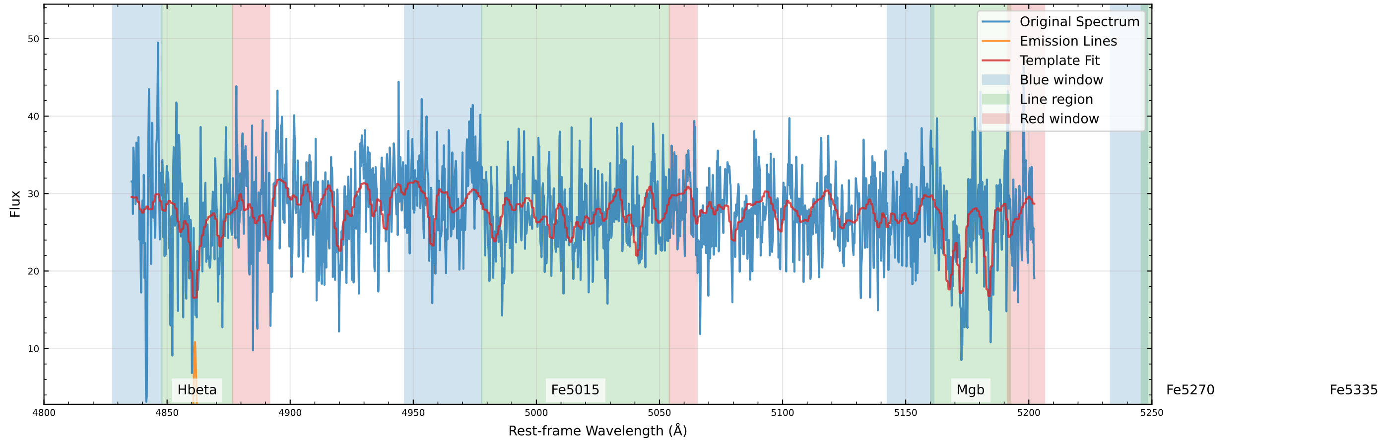
Original Data Comparison ( v_{\text{star}}=50.7 km/s, v_{\text{gas}}=139.0 km/s)
