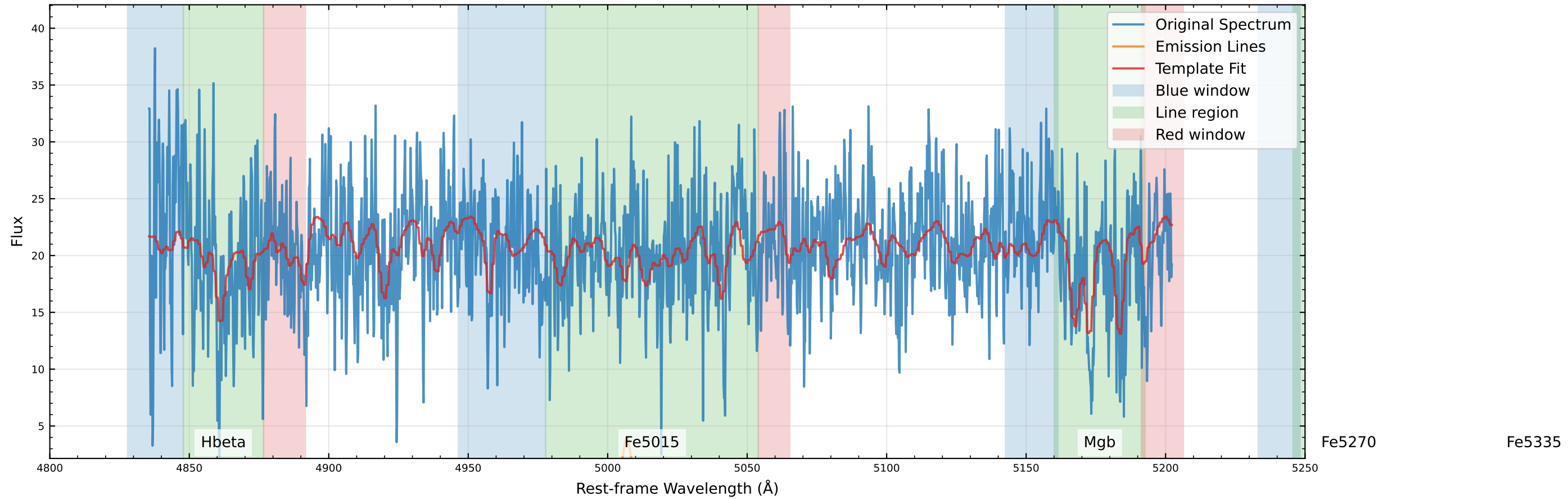
Original Data Comparison (v_star=26.2 km/s, v_gas=53.5 km/s)
