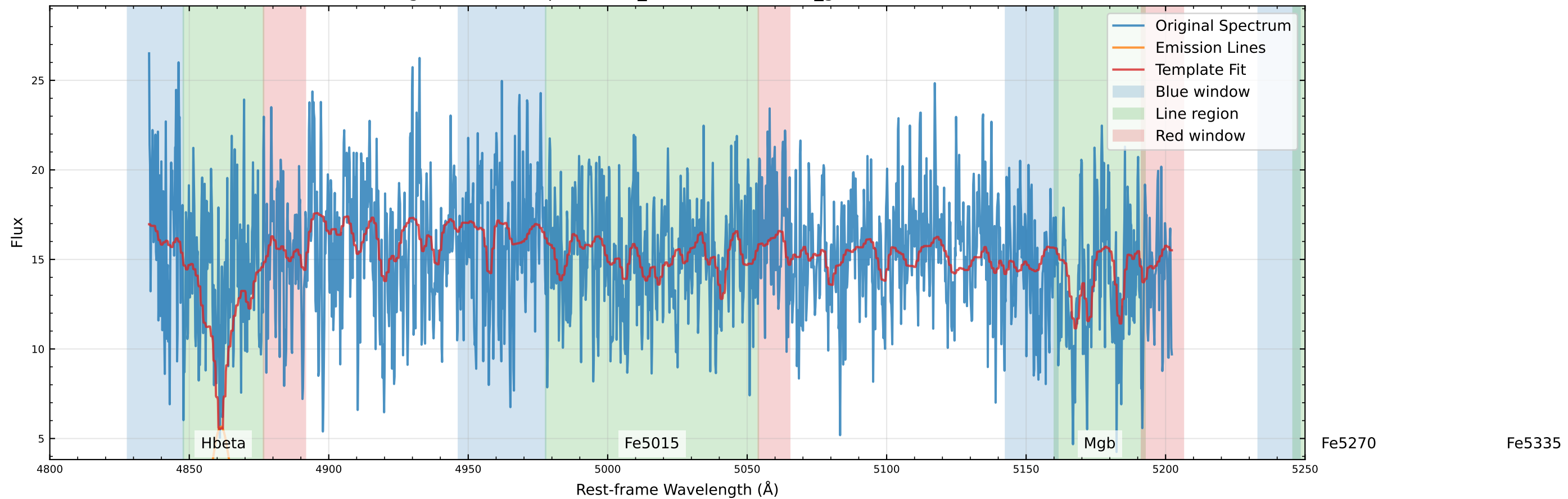
Original Data Comparison ( v_{\text{star}}=-24.2 km/s, v_{\text{gas}}=-70.9 km/s)
