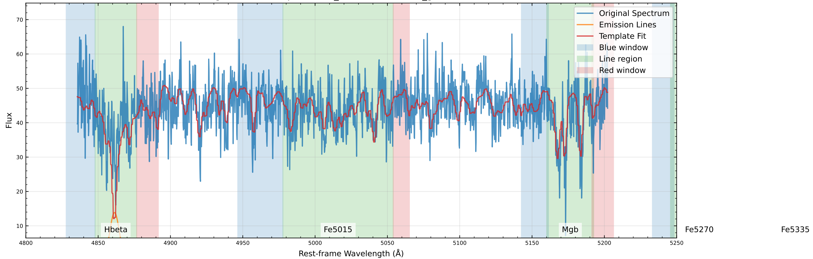
Original Data Comparison (v_star=22.8 km/s, v_gas=81.2 km/s)
