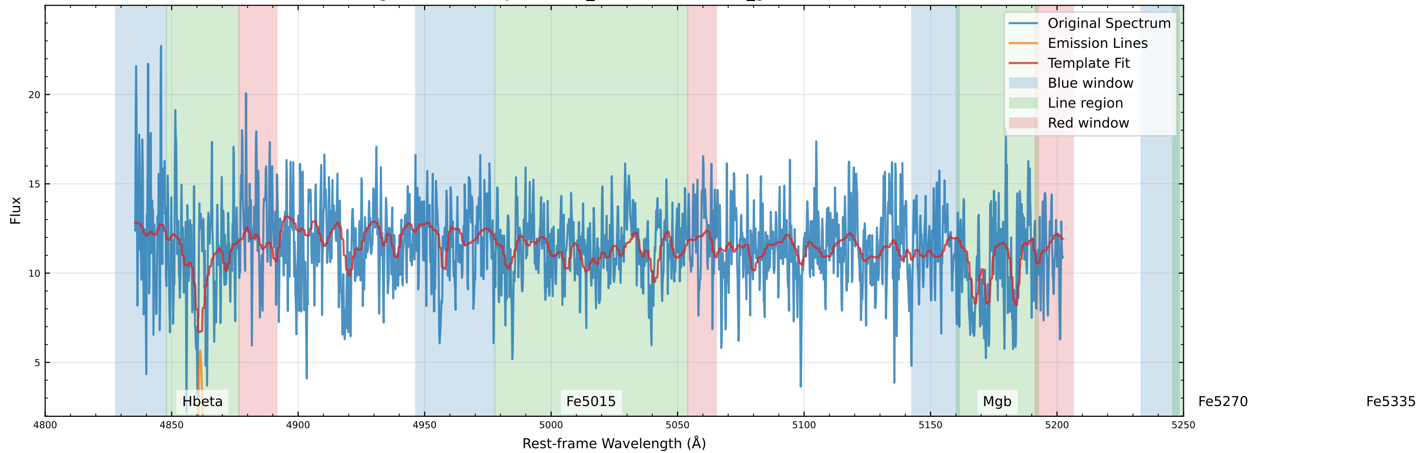
Original Data Comparison (v_star=-64.9 km/s, v_gas=7.9 km/s)
