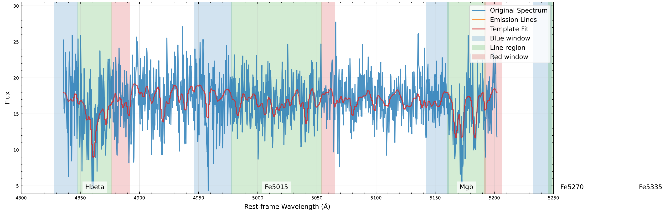
Original Data Comparison (v_star=2.7 km/s, v_gas=49.9 km/s)
