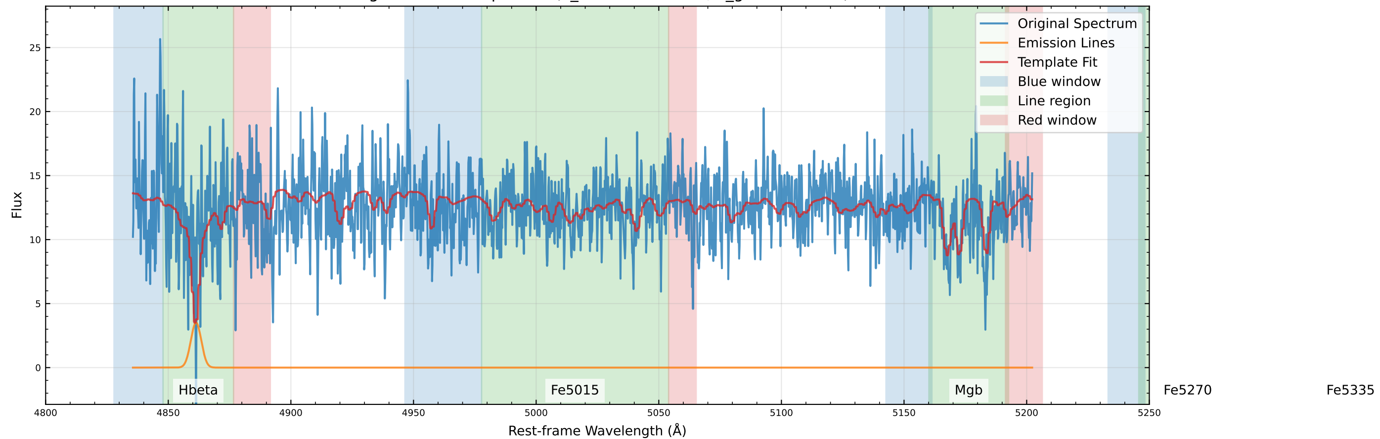
Original Data Comparison (v_star=-15.0 km/s, v_gas=2.9 km/s)
