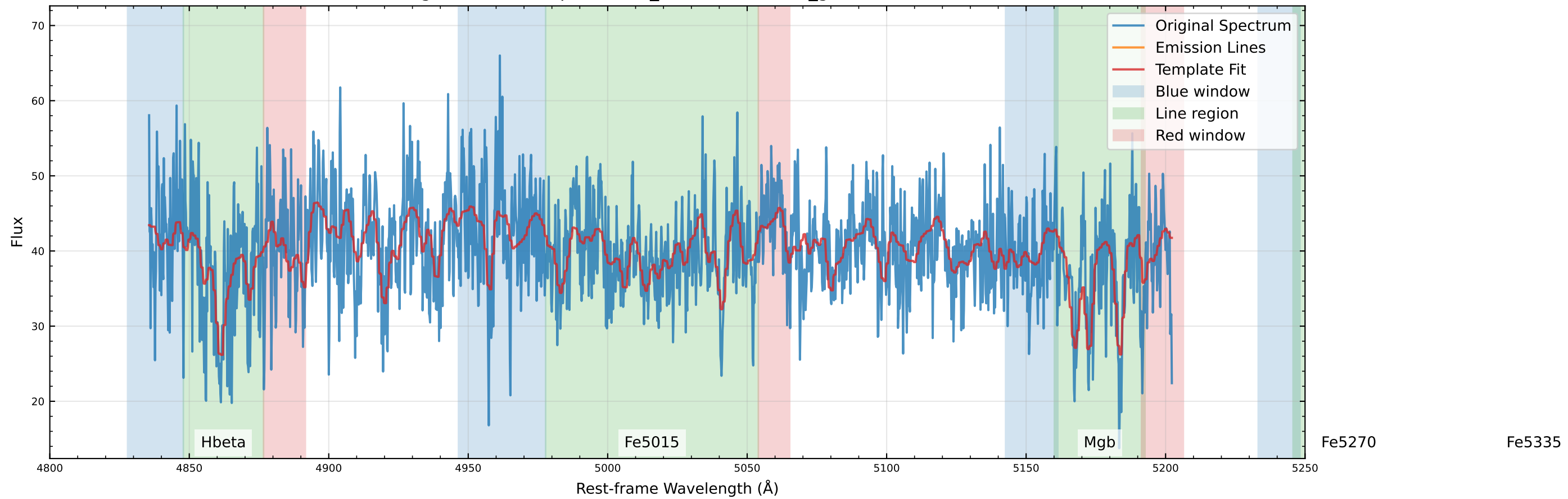
Original Data Comparison (v_star=1.6 km/s, v_gas=82.0 km/s)
