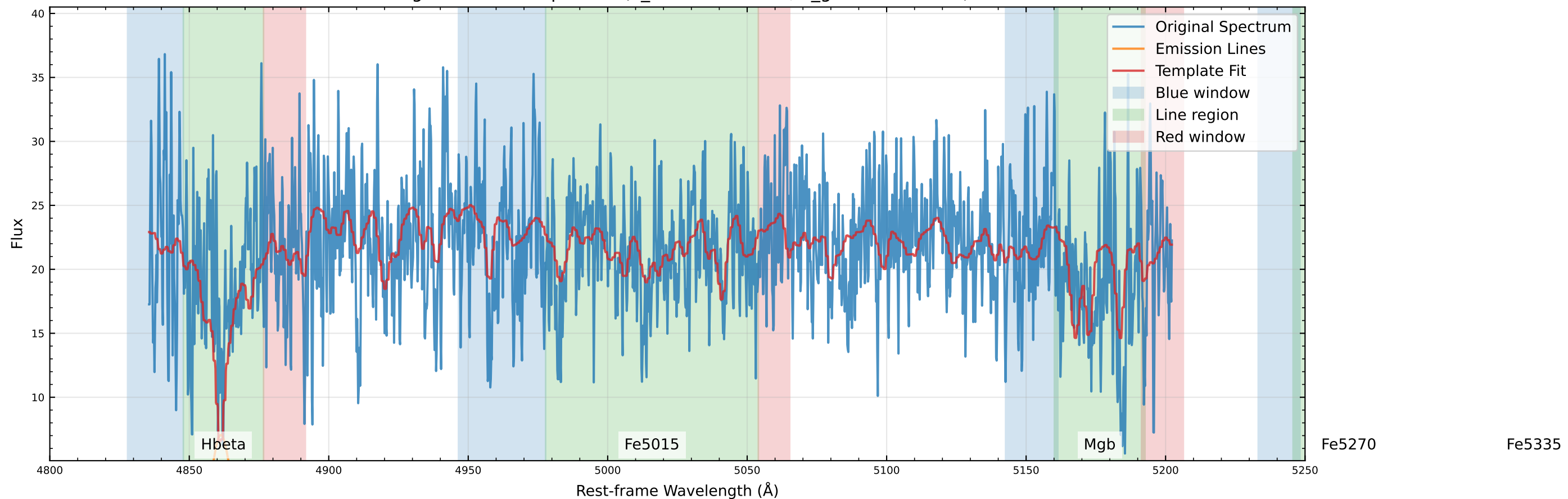
Original Data Comparison (v_star=29.8 km/s, v_gas=-85.4 km/s)
