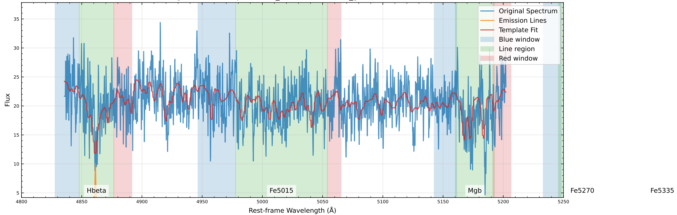
Original Data Comparison (v_star=80.1 km/s, v_gas=159.0 km/s)
