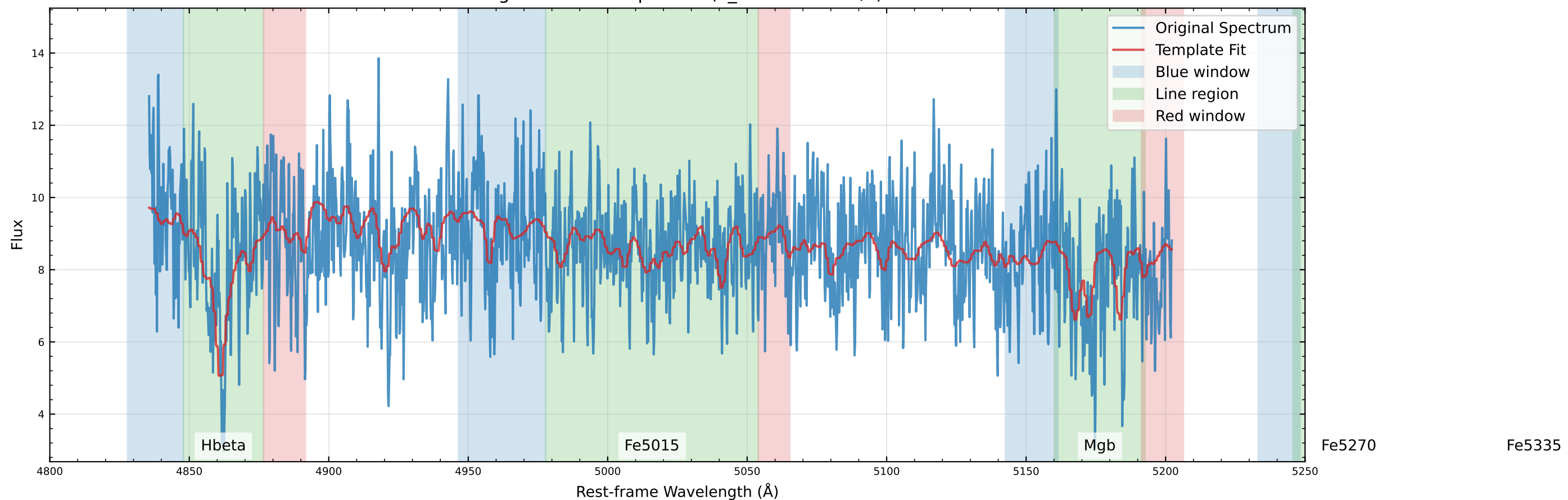
Original Data Comparison (v_star=59.6 km/s)
