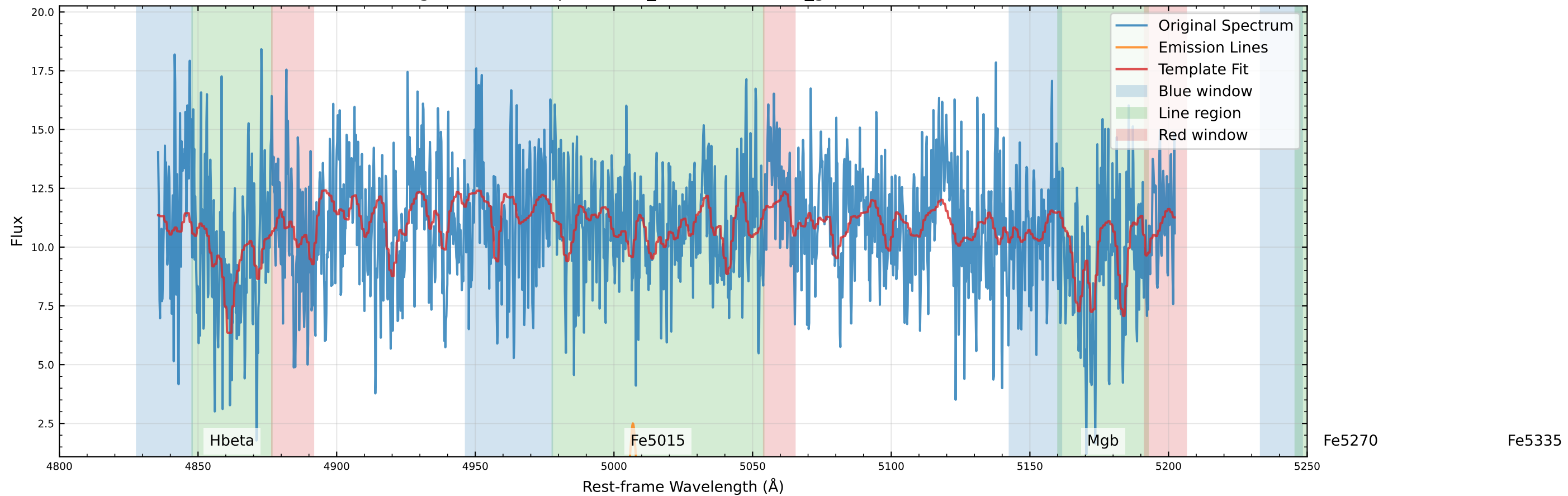
Original Data Comparison (v_star=9.3 km/s, v_gas=-124.6 km/s)
