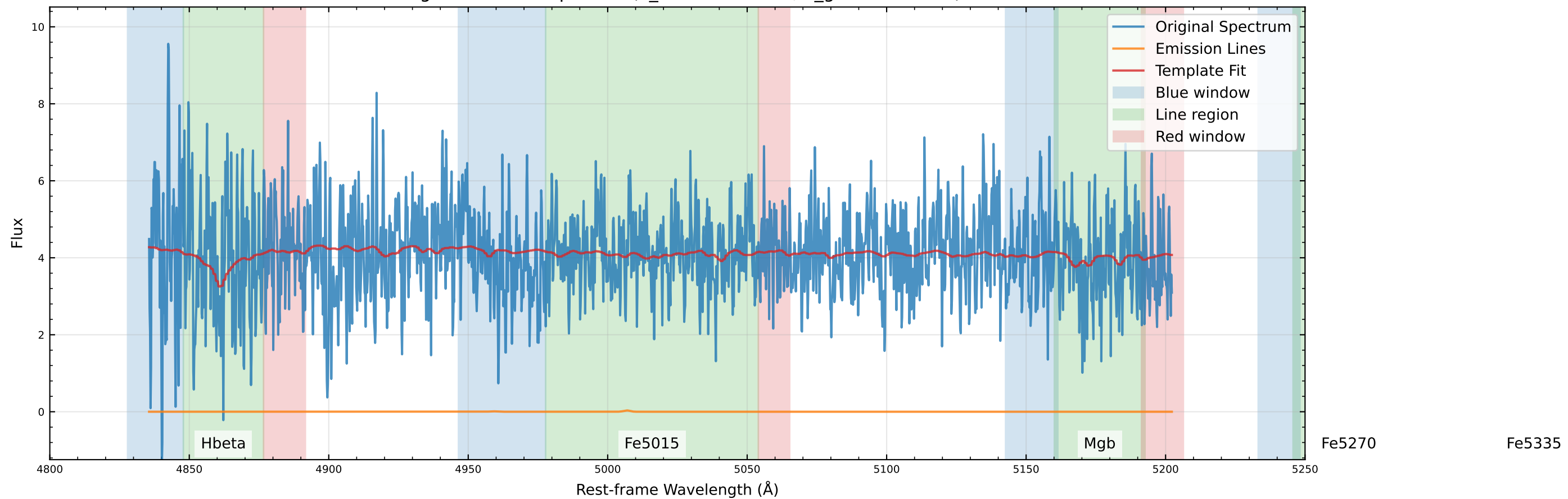
Original Data Comparison (v_star=-1.9 km/s, v_gas=-7.5 km/s)
