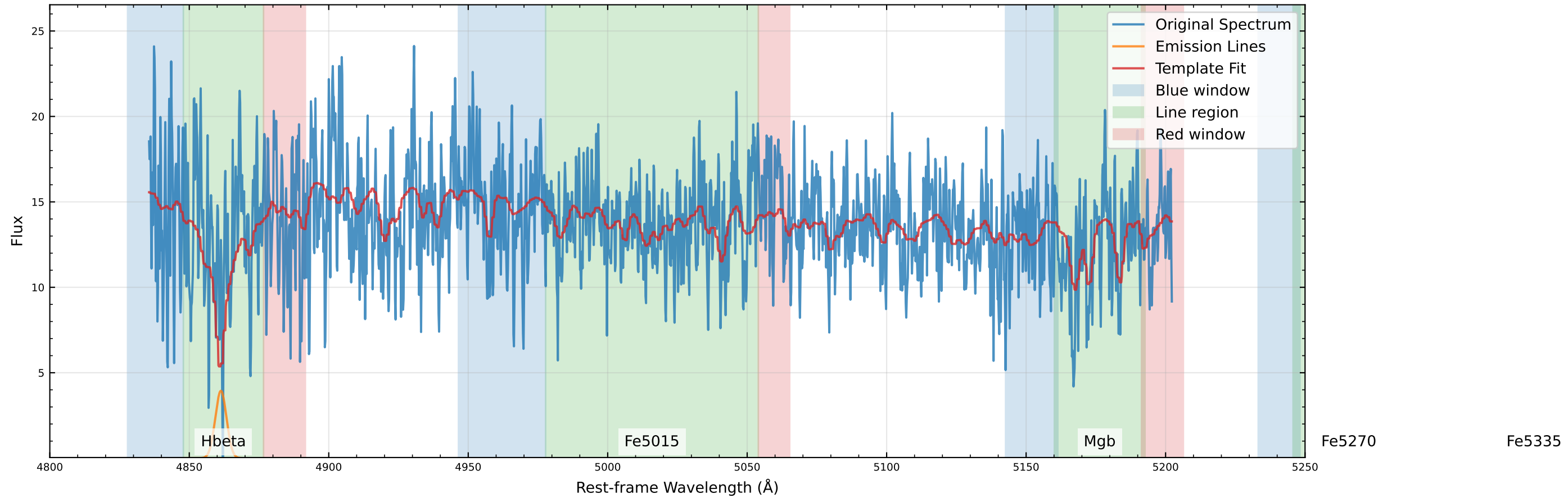
Original Data Comparison (v_star=-19.6 km/s, v_gas=-63.2 km/s)
