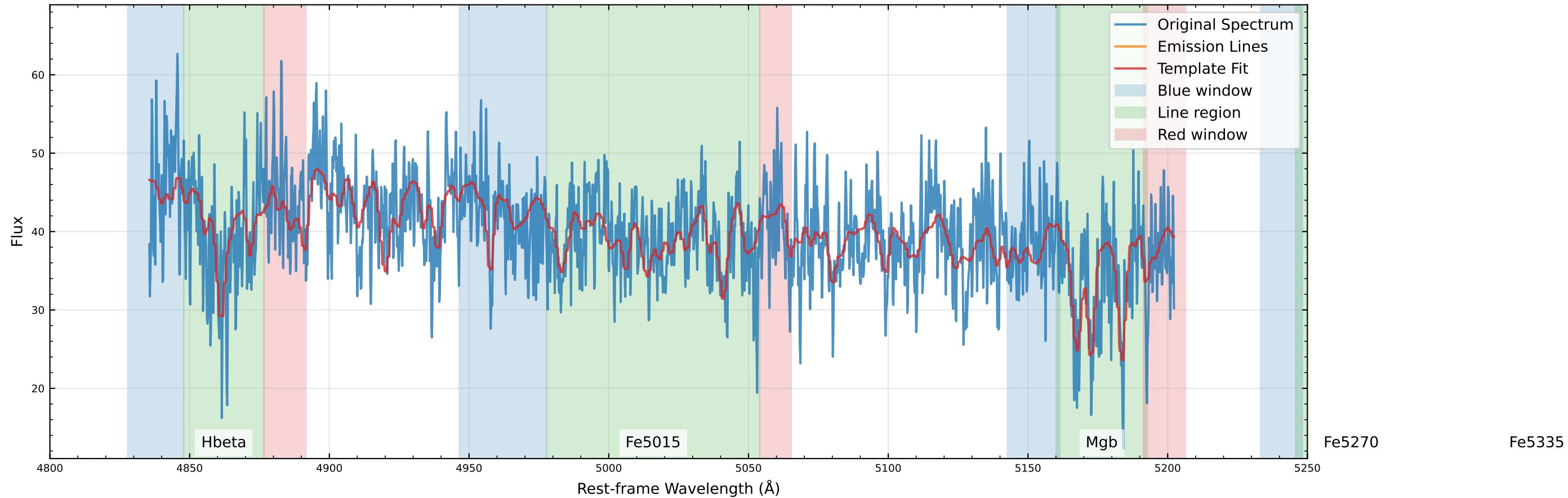
Original Data Comparison (v_star=7.4 km/s, v_gas=36.6 km/s)
