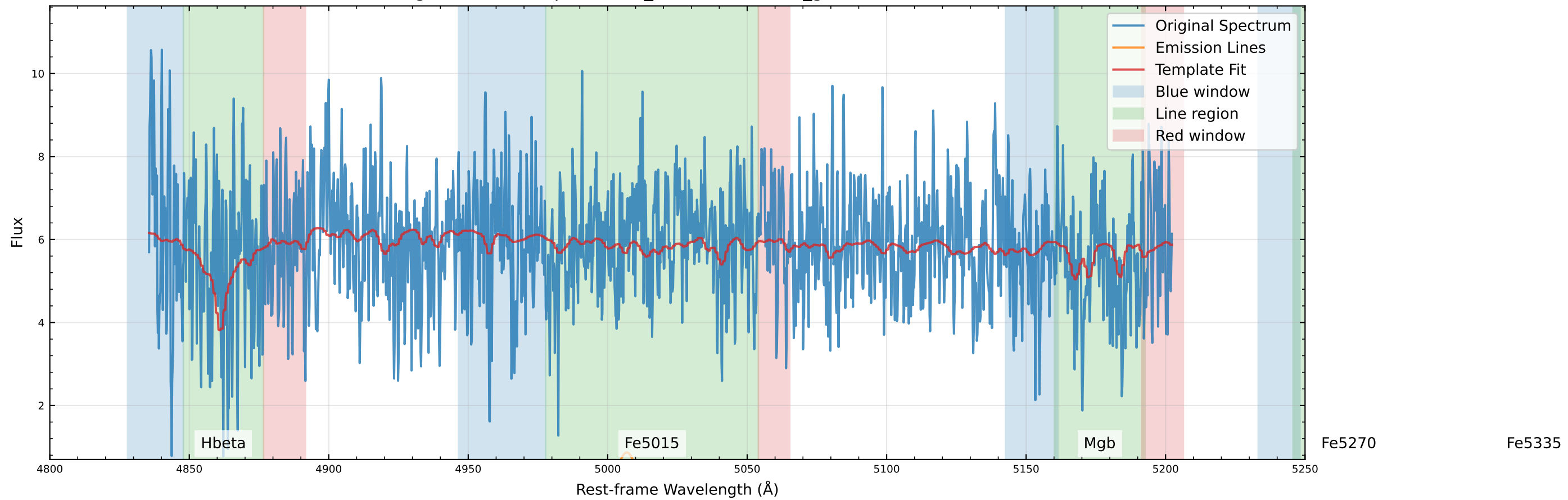
Original Data Comparison (v_star=8.9 km/s, v_gas=210.2 km/s)
