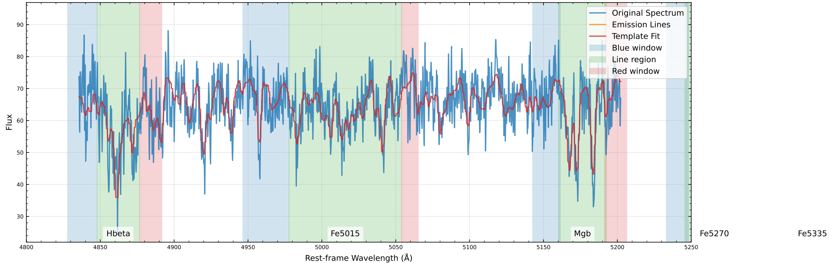
Original Data Comparison (v_star=11.0 km/s, v_gas=60.5 km/s)
