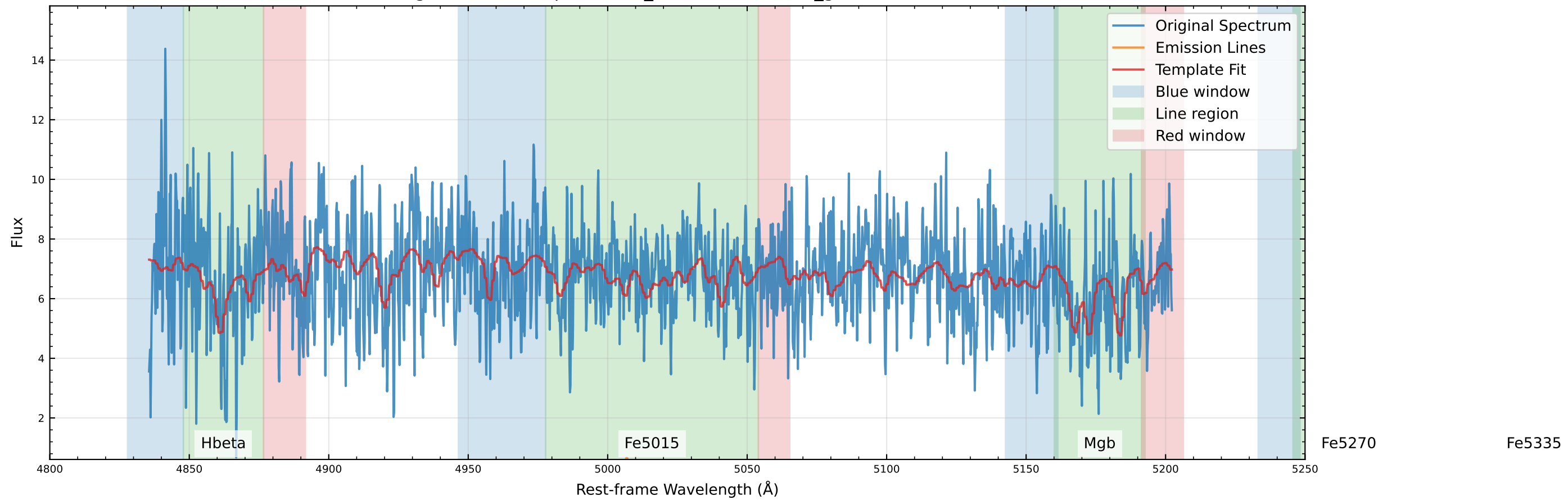
Original Data Comparison (v_star=74.7 km/s, v_gas=24.9 km/s)
